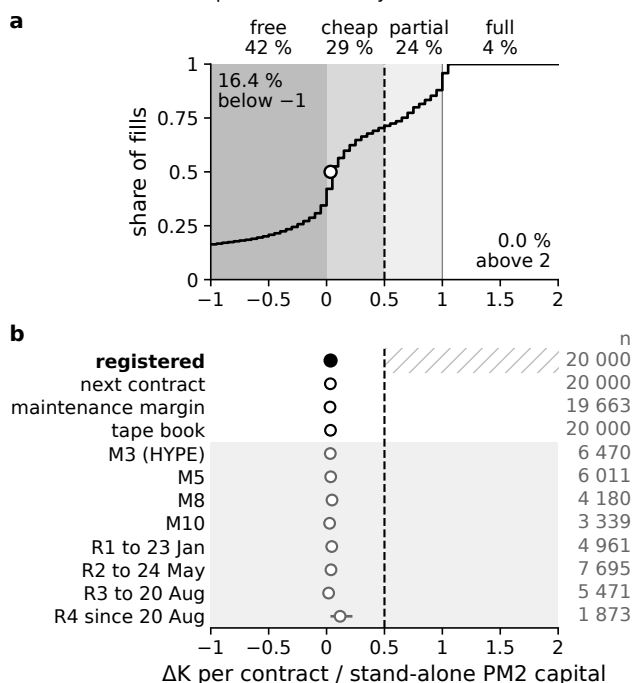
Figure 5: A fill in a dominant maker's book (H2). Panel a is the cumulative distribution of the marginal capital of a fill per contract over its stand-alone PM2 capital, \Delta K/K_{\text{single}} , for the 20 000 tested fills of the four PM2 subaccounts, which trade ETH and HYPE only; the numbers above the bands are the shares of fills in each band, and the shares beyond the axis are given at both ends. The dashed line is the registered threshold of one half, and the circle at height one half is the median; its 90 per cent day-cluster interval is narrower than the circle and printed at the top. Panel b repeats the registered row above the sensitivities and, on grey, exploratory rows per subaccount and per parameter regime. The hatched stretch of the registered row, right of the threshold, is the rejection region: the rule rejects H2 if the interval reaches into it. A maker who starts from an empty book pays the stand-alone capital of Figure 3.
