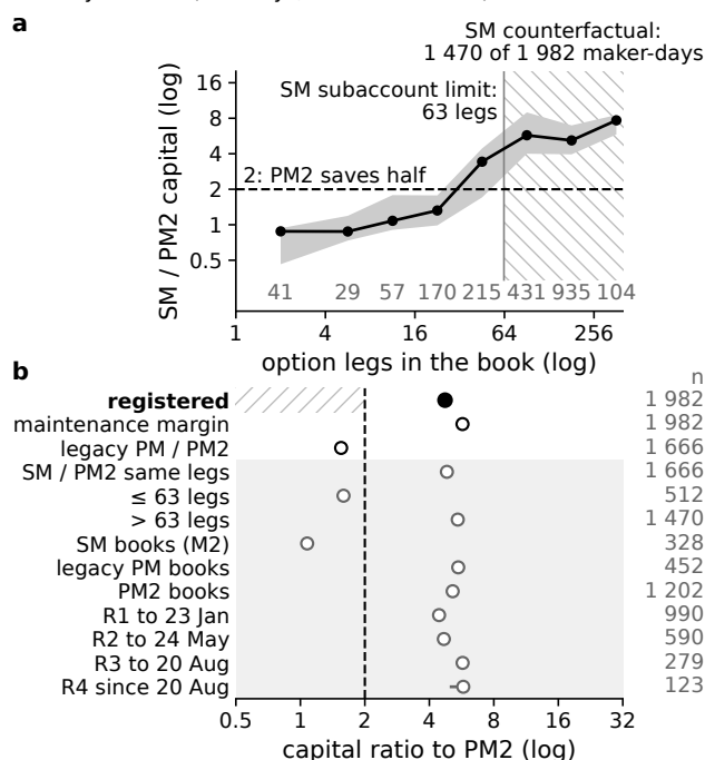
Figure 6: What netting is worth (H3). Panel a is K_{\text{SM}}/K_{\text{PM2}} for the opening books of 1 982 maker-days against the number of option legs, as the median per bin with the interquartile band; the grey numbers above the axis are the maker-days per bin. Beyond 63 legs, the most the endpoint accepted for a standard-margin subaccount in the probes, K_{\text{SM}} is counterfactual (hatched); this is the case on 1 470 maker-days. The dashed line is the registered threshold of two. Panel b is the registered median with its 90 per cent interval, the sensitivities including the legacy manager on BTC and ETH legs, and, on grey, exploratory rows: SM against PM2 on the same BTC and ETH legs, by book size, by the manager of the subaccount and by parameter regime. The hatched stretch of the registered row, left of the threshold, is the rejection region: the rule rejects H3 if the interval reaches into it.
